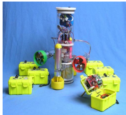
Figure 2: Group photo of the underwater sensor nodes. (a) the static sensor nodes (Aquaflecks) and a mobile node (Amour AUV) [4].
