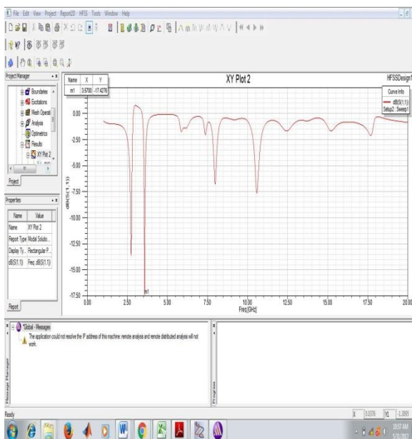
Fig. 3: Return loss of antenna
