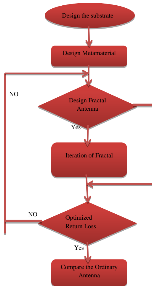
Fig. 1: Proposed Methodology
