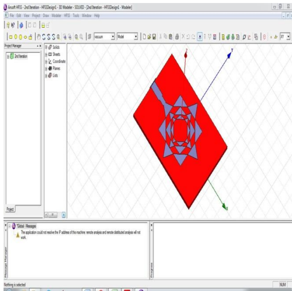
Fig. 2: Fractal Antenna design with Metamaterial Substrates
